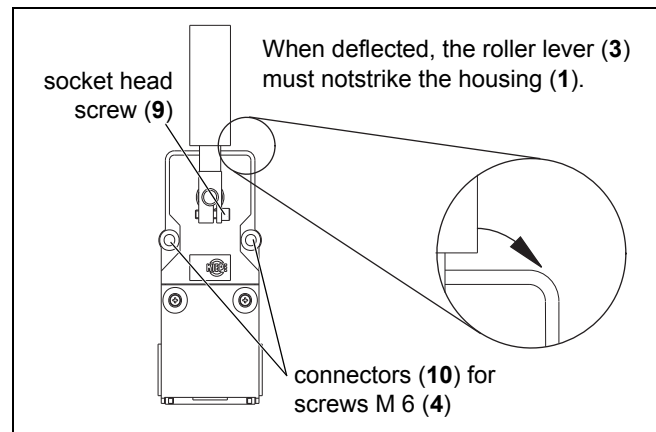
Fig. 7-1: Misalignment switch: Replace roller levers
