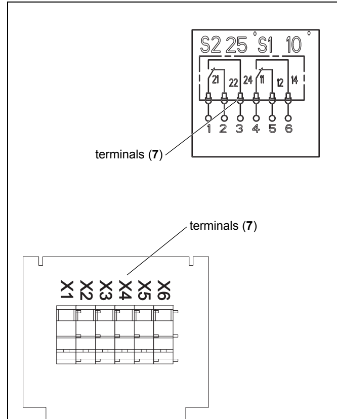
Fig. 5-6: Configuration of the terminals
