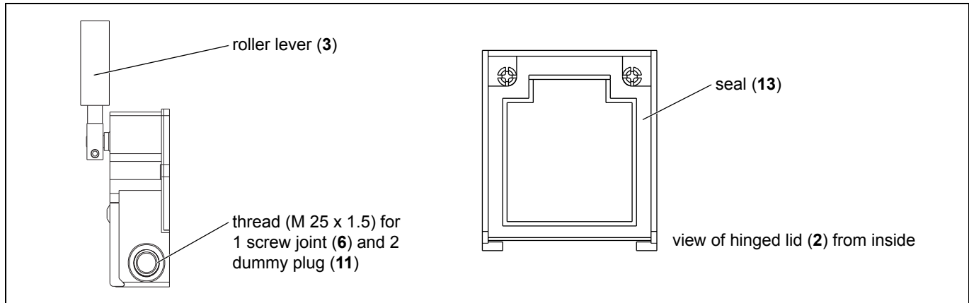
Fig. 8-2: Replacement parts
