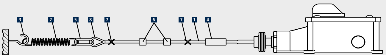
Single-sided pull rope installation
